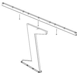
Fig. 10. Method of mounting Steel Profile A to the vertical support
