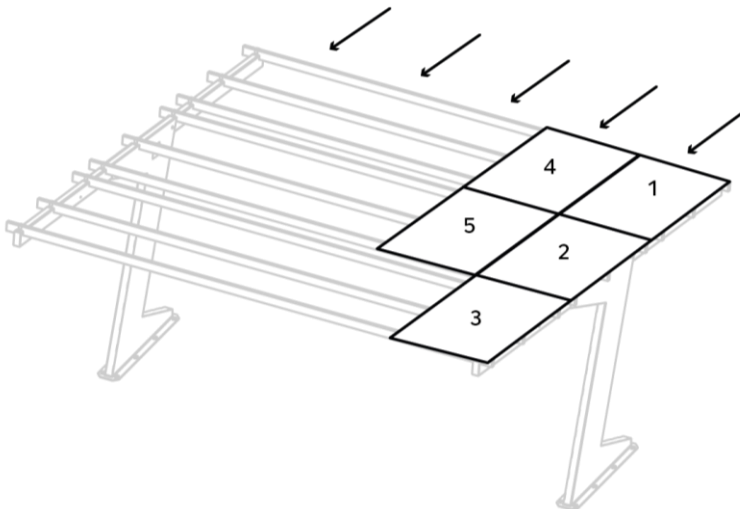
Fig. 21. Correct sequence for mounting modules on the structure.
