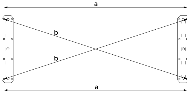
Fig. 5. The diagonals and distances that should be aligned when positioning the steel brand
