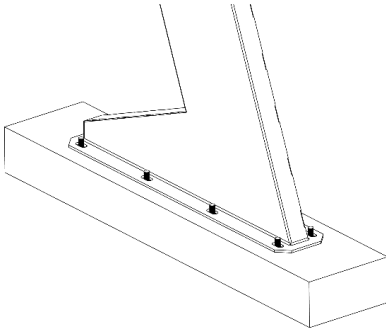
Fig. 8. Installation of the vertical support on the foundation
