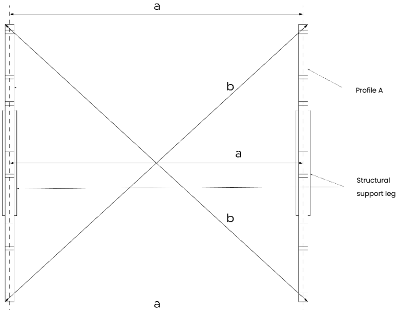
Fig. 14. Diagonals and distances that should be aligned after placing Steel Profile A.
