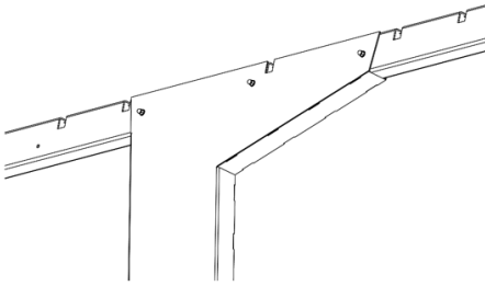
Fig.13. Correct fastening of Profile A with the vertical support
