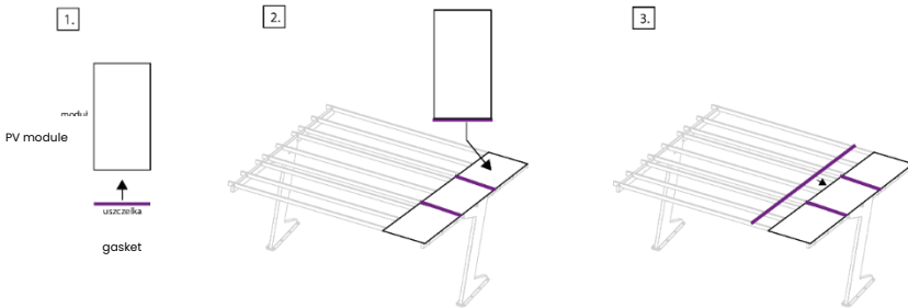
Fig. 25. Proper method for installing gaskets on photovoltaic modules:
