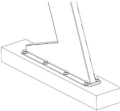
Fig. 9. Screwing the vertical support to the foundation base
