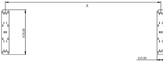
Fig. 4. Arrangement of the steel brands for mounting the Avrii SOL Integra carport
