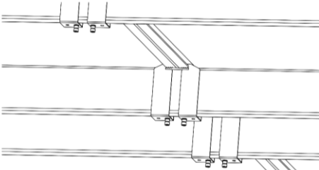
Fig. 24. Mounting the modules to the carport structure
