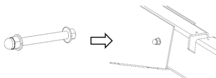
Fig. 12. Preparation and installation of Profile A with the vertical support
