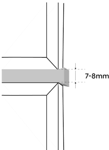
Fig. 23. Proper pressing of the gasket between the modules
