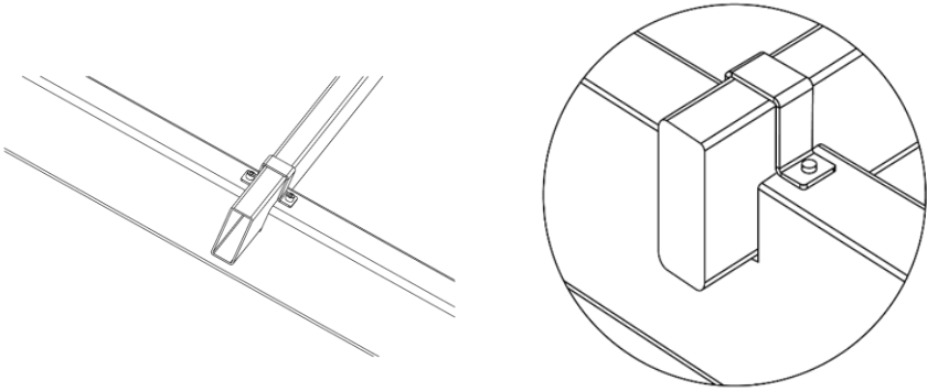
Fig. 15. Attaching Profile B to Profile A
