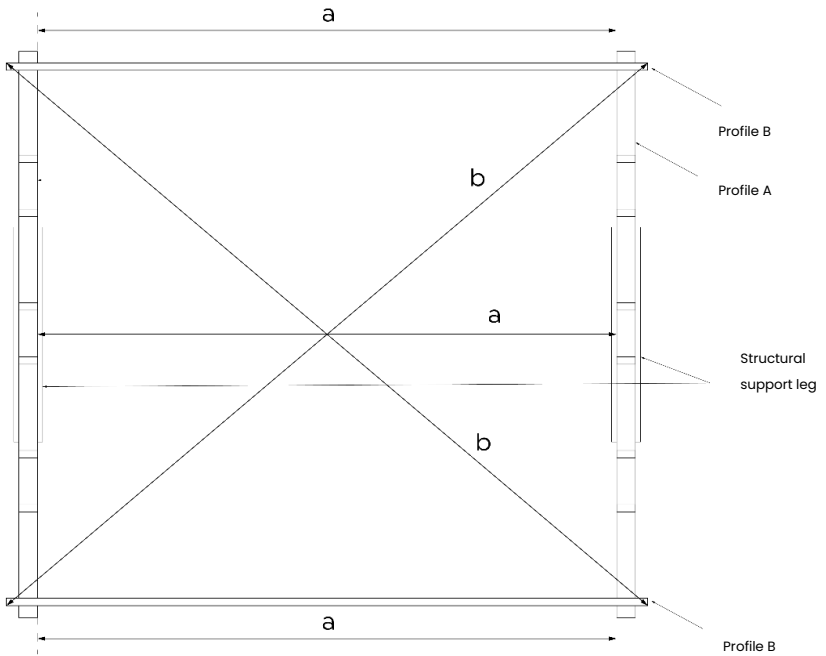
Fig. 16. Diagonals and distances that must align after positioning Profile A and the outer Profile B elements
