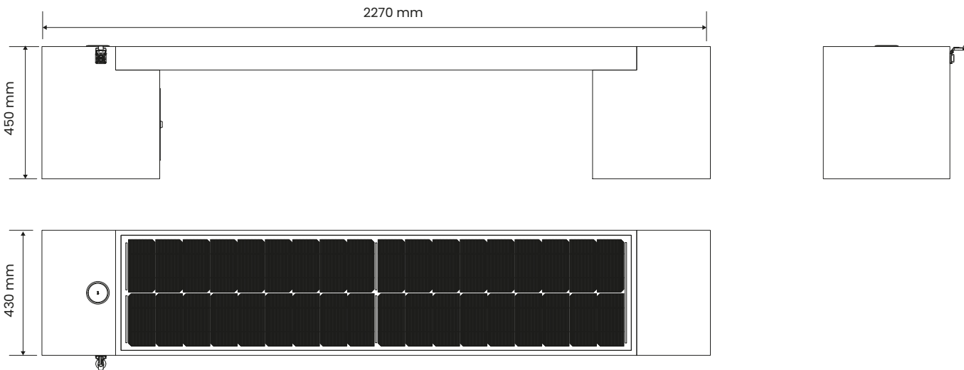
Avrii INTEGRA photovoltaic bench – technical drawing
